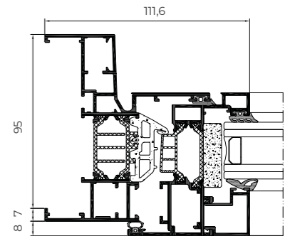
* COR 70 OC Half Hidden sash - Mitred frame
