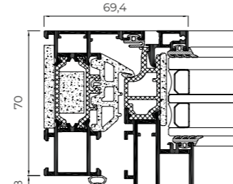
Cor 70 Industrial - Half-Hidden Sash
